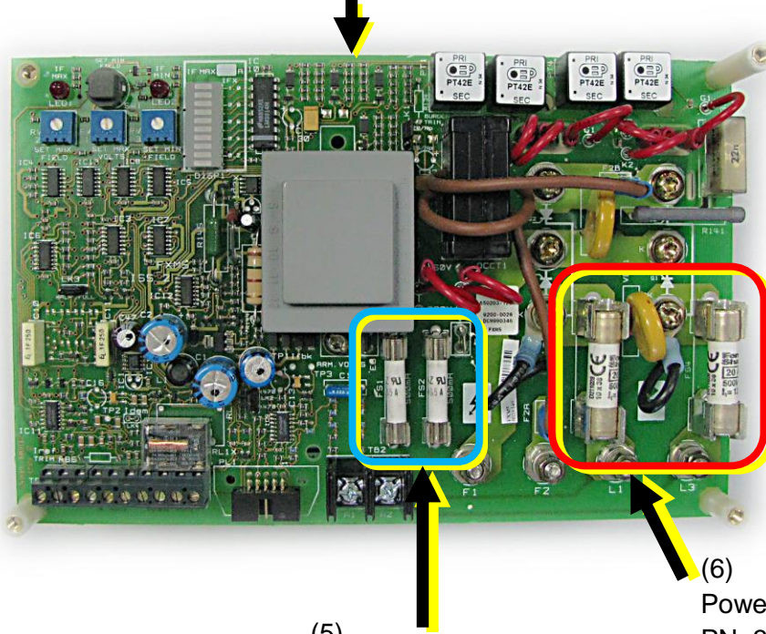
(5) Control Fuses PN: 3537-3251
